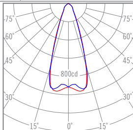
06992 - LENS "SQUARE"
