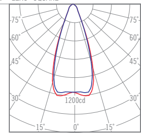
06997 LENS "SQUARE"
