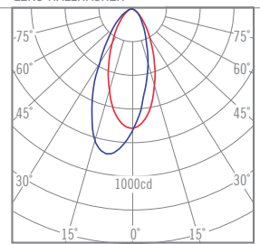
06996 LENS WALLWASHER
