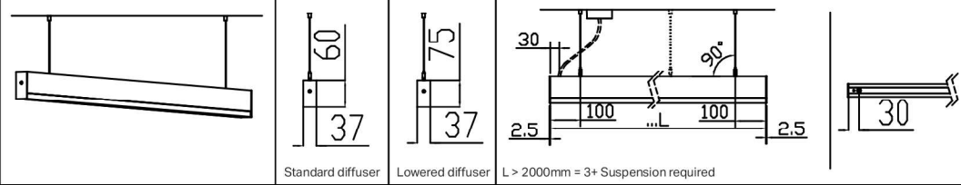
Standard diffuser Lowered diffuser L > 2000mm = 3+ Suspension required
